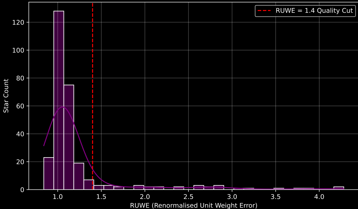
GALAH DR4 Field [182] RUWE Distribution (n= 284)
