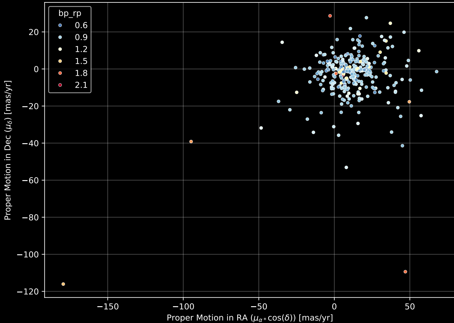
GALAH DR4 Field: [182] Proper Motion Diagram (n= 295)
