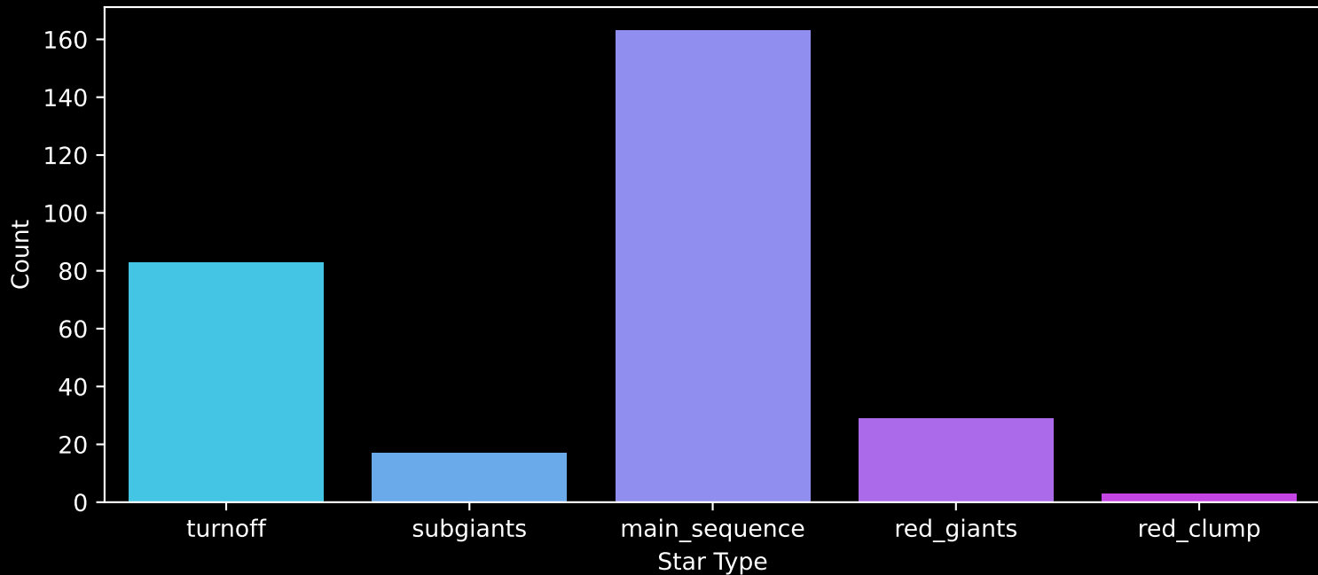
GALAH DR4 Field: [182] Count plot of Star Type
